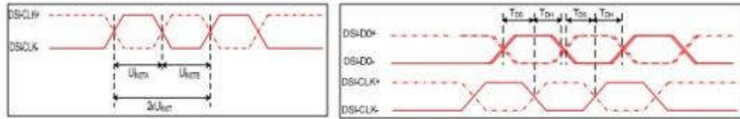
Figure 4.1.1 clock channel timing
