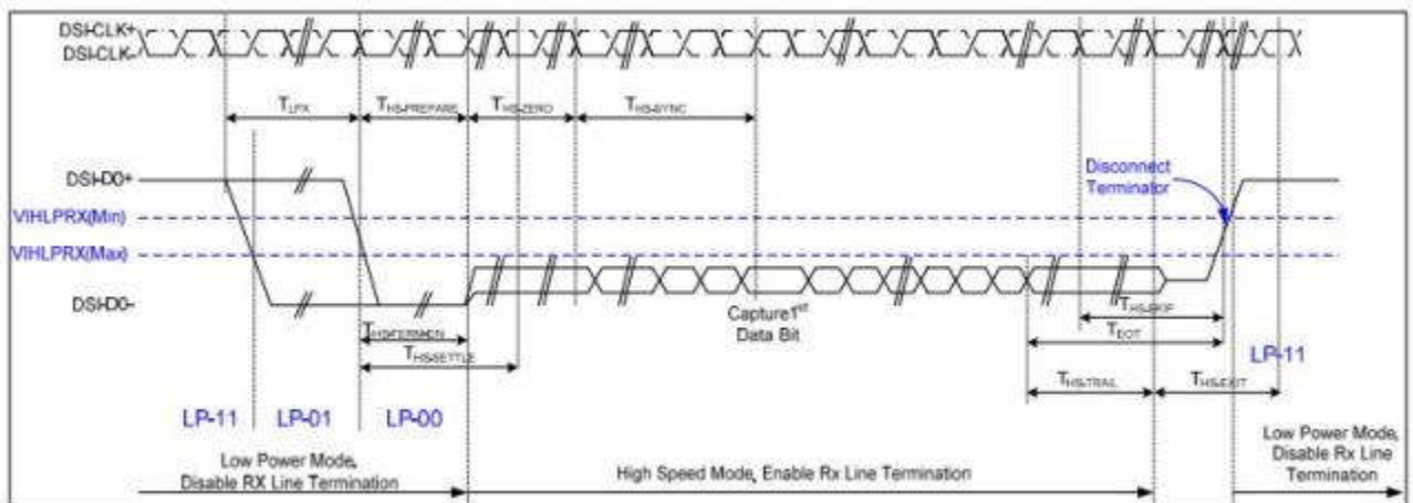
Figure 4.1.3 High speed data transmission timing sequence
