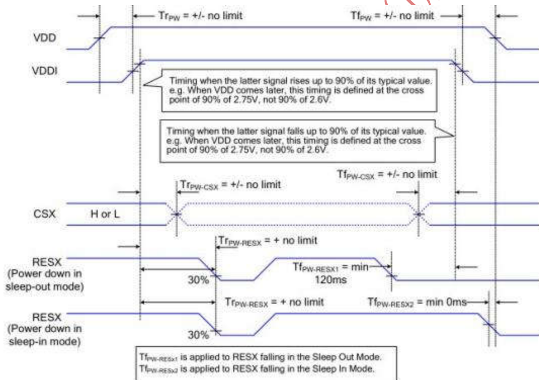
Figure 4.3.1 VCI/VDDI input power off/on sequence
